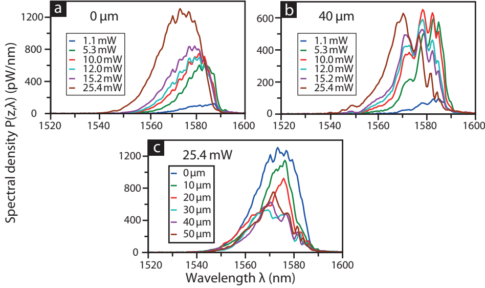
Figure 3.4: Evolution of the shape of the spectral density. A series of spectra taken at the beginning a) and after 40 \mu\text{m} propagation b) in the slow-light PhCW for different average input powers. c) A series of spectra taken in 10 \mu\text{m} steps at an average input power of 25.4 mW.
